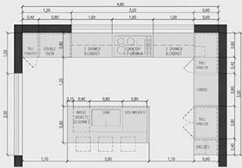
KITCHEN LAYOUT
